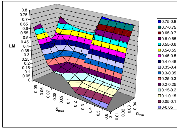
Figure 8: Anonymization cost vs. various values of \delta_{min} and \delta_{max} for the MPALM n2 strategy
