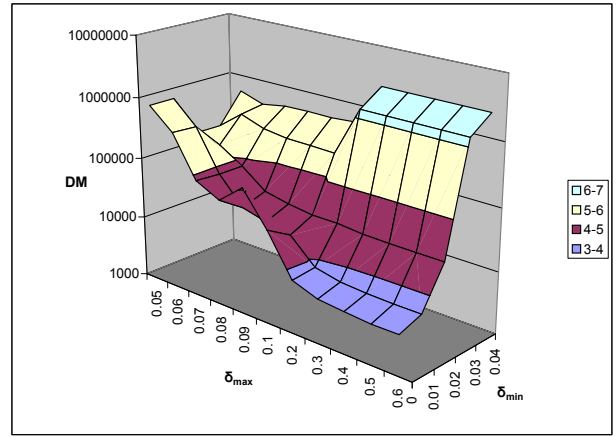
Figure 8: Anonymization cost vs. various values of \delta_{min} and \delta_{max} for the MPALM n2 strategy
